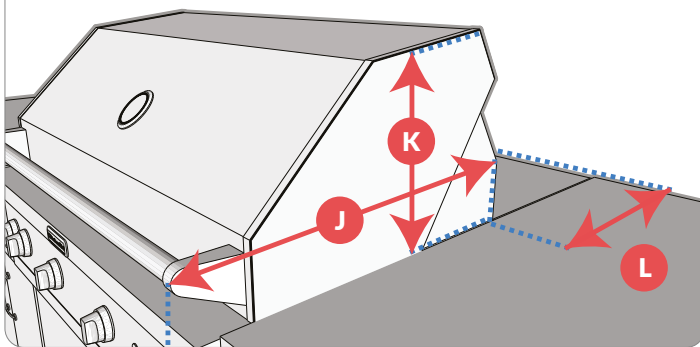
Grill detail
